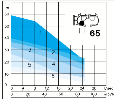
RW40 series
