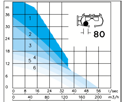
RW40 series
