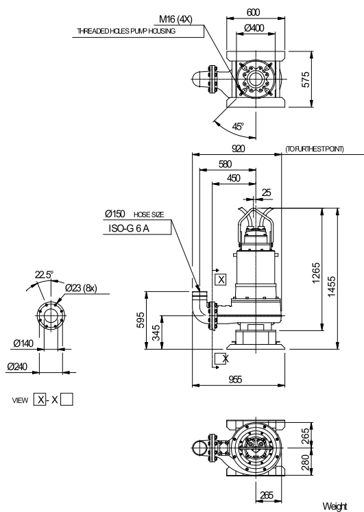
Dimensional drwg CS3201 HT
