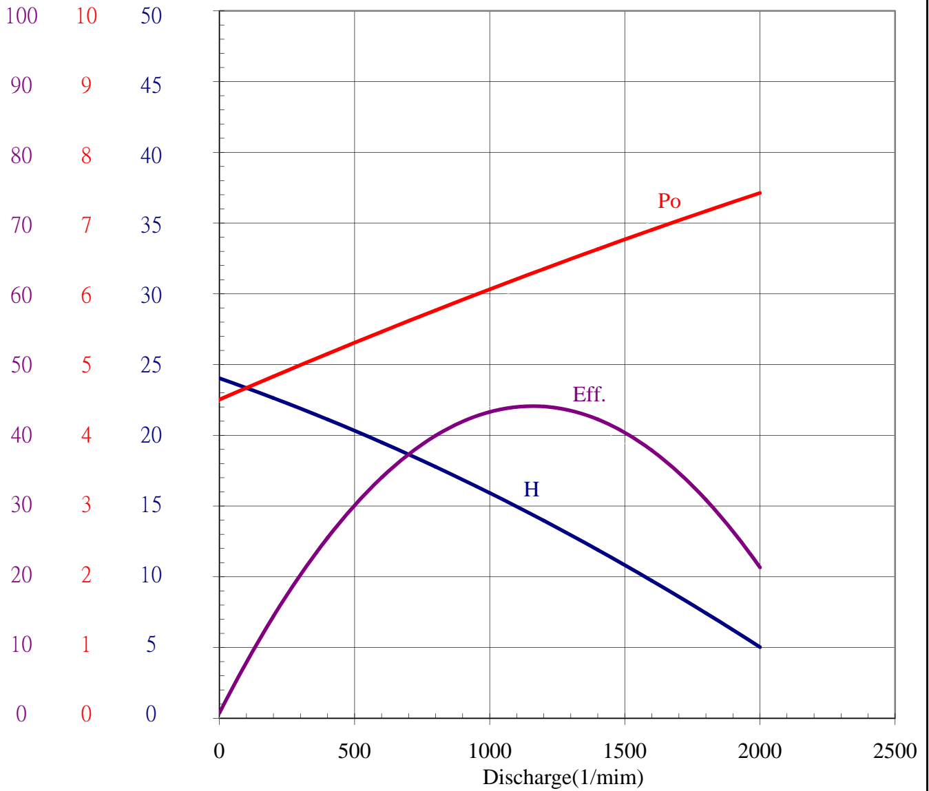
PUMP Performance Curve
