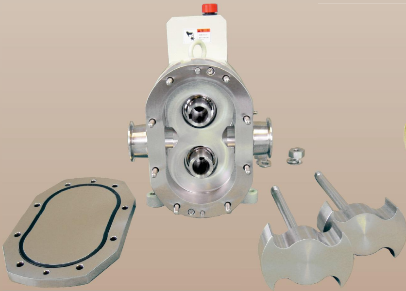
Double blade rotor
