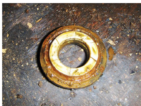
Mechanical Seal, gebroken.
