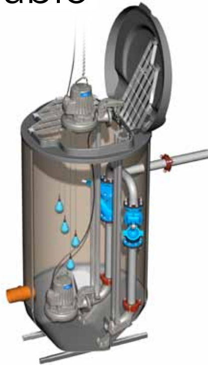
In a two-pump station, four level regulators are generally used. One is positioned at the stop level, one at each pump's start level, and the fourth regulator is used to trigger a high level alarm.
